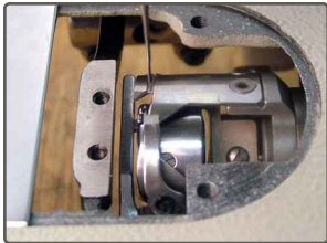
DETAIL OF THREAD TRIMMER KNIVES
