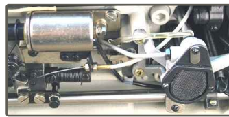
AUTOMATIC OIL LUBRICATION SYSTEM BY PUMP AND THREAD TRIMMER SOLENOID
